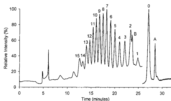
Fig. 1. Mixed-mode HPLC–ESI–MS summed ion chromatogram of a sediment extract (32–36 cm depth core slice) showing resolution of NPEOs and NPs. Numbered peaks correspond to NPEOs and [ ^{13}\text{C}_6 ]NPEOs with the indicated number of ethoxy groups (0=NP, [ ^{13}\text{C}_6 ]NP; 1=NP1EO, [ ^{13}\text{C}_6 ]NP1EO; etc.). Peaks 'A' and 'B' are the internal standards, n -NP and n -NP3EO, respectively. Note the discontinuity at retention time 25.8 min, corresponding to the shift in MS polarity from positive to negative ion mode.
