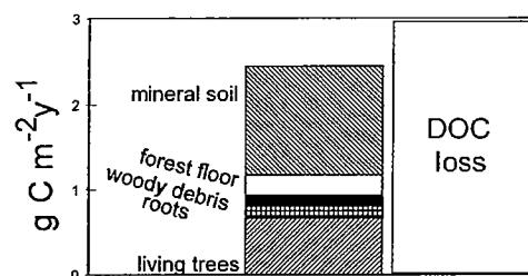
Fig. 1. Loss and net accumulation of organic C for an undisturbed watershed at the Hubbard Brook Experimental Forest in New Hampshire, USA. Data from Gosz et al. (1978), Likens et al. (1977), Bormann and Likens (1979) and McDowell and Likens (1988). DOC is not the only form of organic matter lost from the forest; thus, the loss term is an underestimate of true loss.
