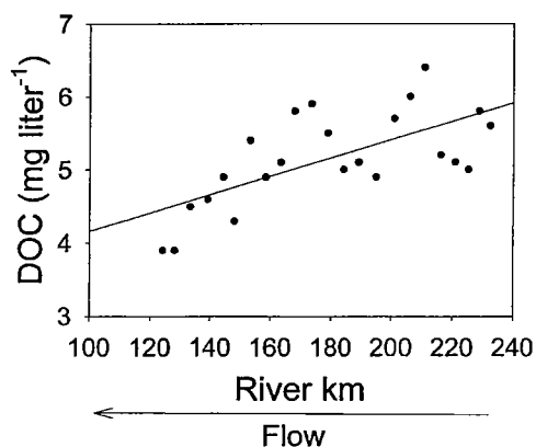
Fig. 4. DOC concentrations along a longitudinal transect in the Hudson River. River km (X-axis) is distance along the river that flows from the north (Albany, NY; river km 245) towards New York City (river km 0). Slope of regression line, 0.012 mg C L -1 km -1 — consistent with a loss term of ~100 g C m -2 year -1 of allochthonous organic C. The line is significant ( P < 0.01 ) but the r^2 low 0.44, so the data generate a range of loss terms from 85 to 185 g C m -2 year -1 .
