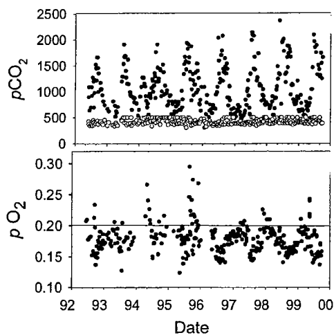
Fig. 3. Direct measurements in the Hudson River at weekly intervals, 1992–1999. (upper) partial pressure of \text{CO}_2 ( p\text{CO}_2 ): ● in the surface water; ○ in the overlying atmosphere (lower) partial pressure of \text{O}_2 ( p\text{O}_2 ): ● in the surface water; solid line, in the atmosphere.
