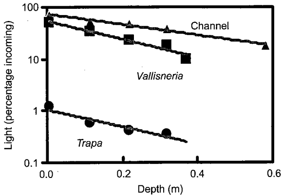
FIG. 4. Measured light over depth in the channel (triangles), Vallisneria bed (squares), and Trapa bed (circles), expressed as a percentage of incoming photon flux. The lines represent the fit exponential equations. Note the log scale.
