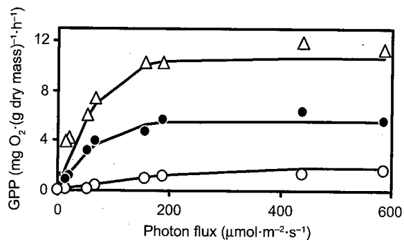
FIG. 3. Gross primary production (GPP) vs. light for Vallisneria leaves (triangles), Trapa feather leaves (solid circles), and Trapa rosette leaves (open circles). Each point is the mean of three replicates, and the cv of points averaged 5% of the mean. Photon flux values extended to 2000 \mu\text{mol}\cdot\text{m}^{-2}\cdot\text{s}^{-1} , but we show values only to 600 \mu\text{mol}\cdot\text{m}^{-2}\cdot\text{s}^{-1} so that response at low light can be better seen. The lines are a hyperbolic tangent fit to all data. For Vallisneria , Trapa feather, and Trapa rosette leaves, modeled vs. measured GPP agreed well ( r^2 = 0.96, 0.97, and 0.96, respectively).
