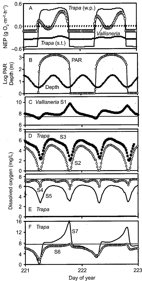
FIG. 9. Output of model for two days in July 2000. (A) Hourly net ecosystem production (NEP) for Vallisneria beds (open circles), Trapa beds including floating leaves (labeled Trapa (w.p.) [whole plant]), and for submersed Trapa tissue only (labeled Trapa (s.t.)). (B) Modeled incoming photosynthetically active radiation (PAR, open circles) and tidal variation in water column depth. Panels C–F show modeled DO for different model scenarios (S1–S7) described in Table 2. (C) Modeled DO variation in Vallisneria beds compared to a mean value of 7.5 mg/L in the channel (gray line). (D–F) Modeled DO variation in the Trapa bed for six different scenario runs (Table 2). Note that S1, S2, and S3 correspond well to actual measured DO dynamics in Vallisneria and at the inner and edge sites and the Trapa bed, respectively (Fig. 6).
