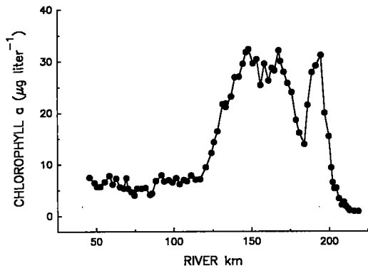
Fig. 7. Spatial variation in Chl a concentration along the length of the tidal freshwater river in August 1991. Samples were taken over the course of 2 d. River km are kilometers upstream from Battery Park (0).
