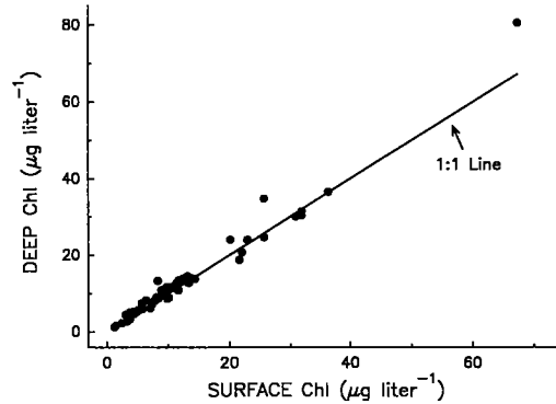
Fig. 2. Concentration of Chl a in samples of surface water plotted against samples from deep water. Surface samples were always collected at 0.5 m below the surface; deep samples were collected at least 1 m above the sediments. Depth of the deep samples varied from 5 m to >10 m depending on station depth (see Fig. 10). The 1:1 line (surface Chl = deep Chl) is shown for comparison.
