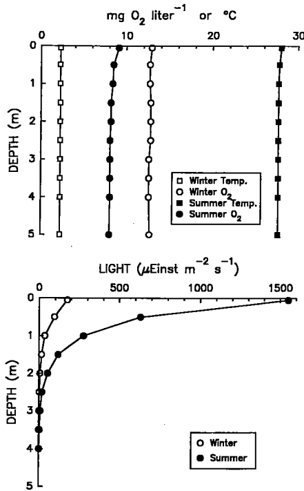
Fig. 1. Representative profiles of temperature, dissolved oxygen, and light (at midday) for winter and summer conditions in the Hudson River.
