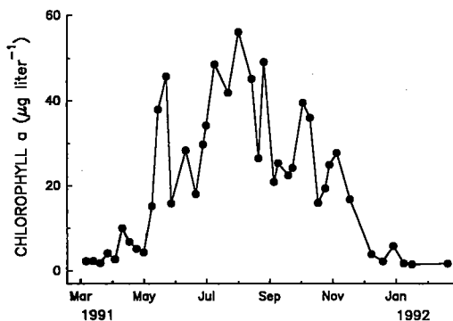
Fig. 6. Seasonal cycle of Chl a concentrations from a single station (Rhinecliff), March 1991 through February 1992.
