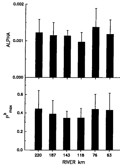
Fig. 3. Longitudinal variation in \alpha and P_{\text{max}}^b . Samples for each station are means of seven dates during the growing season (May–October); error bars represent 95% C.L. Units for \alpha are \mu\text{mol C } (\mu\text{g Chl } a)^{-1} \text{ h}^{-1} (\mu\text{Einst m}^{-2} \text{ s}^{-1})^{-1} ; units for P_{\text{max}}^b are \mu\text{mol C } (\mu\text{g Chl } a)^{-1} \text{ h}^{-1} . River km are kilometers upstream from Battery Park (0).
