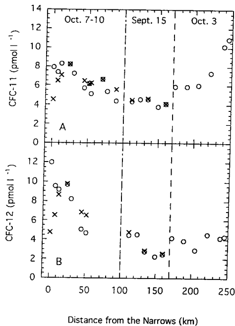
Figure 6. Distribution of CFCs along the axis of the Hudson estuary collected between September 15 and October 10, 1992. On September 15 the saltwater-freshwater interface was about 100 km upstream of the Narrows. Circles indicate surface samples, and crosses indicate bottom samples.
