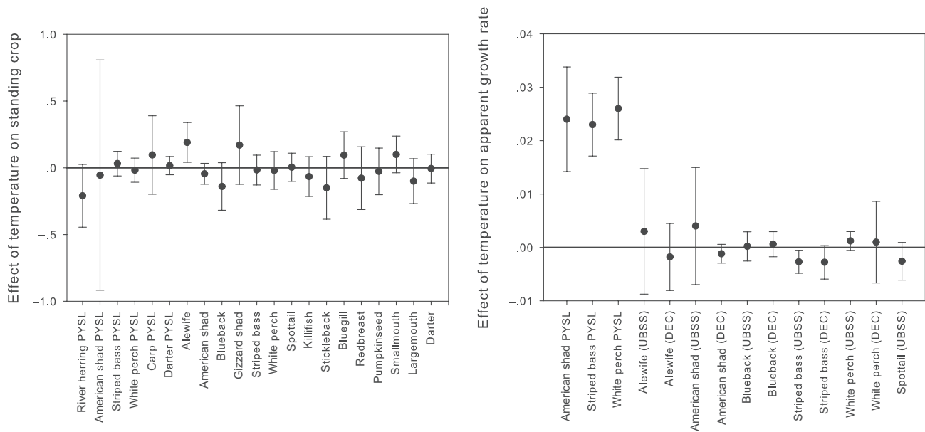
Figure 4. Effects of water temperature on the abundance and growth rates of fishes in the Hudson River, based on Strayer and colleagues (2004). The units are changes in log 10 -transformed abundance per degree Celsius and changes in growth rate (per week) per degree Celsius. The abundance data are from the utilities beach seine survey of juveniles; the growth analysis includes both post-yolk-sac larvae (PYSL) and juveniles, from two independent data sets. See Strayer and colleagues (2004) for details. The error bars represent the 95% confidence intervals. Abbreviations: DEC, New York State Department of Conservation survey; UBSS, utilities beach survey.
