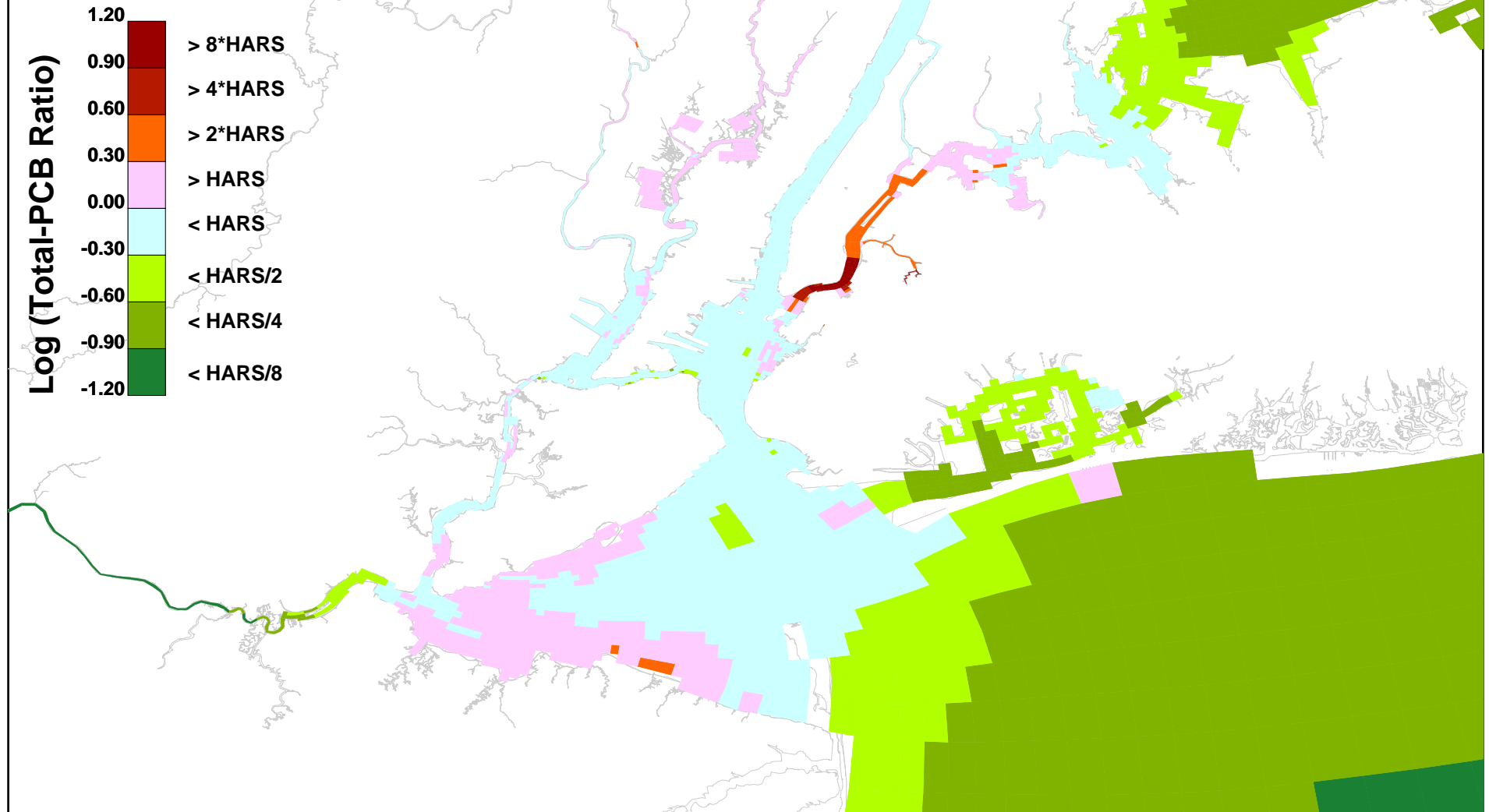
Figure 2. Total-PCB, Sediment Bed Depth Averaged, Calibration, 1998-2002
